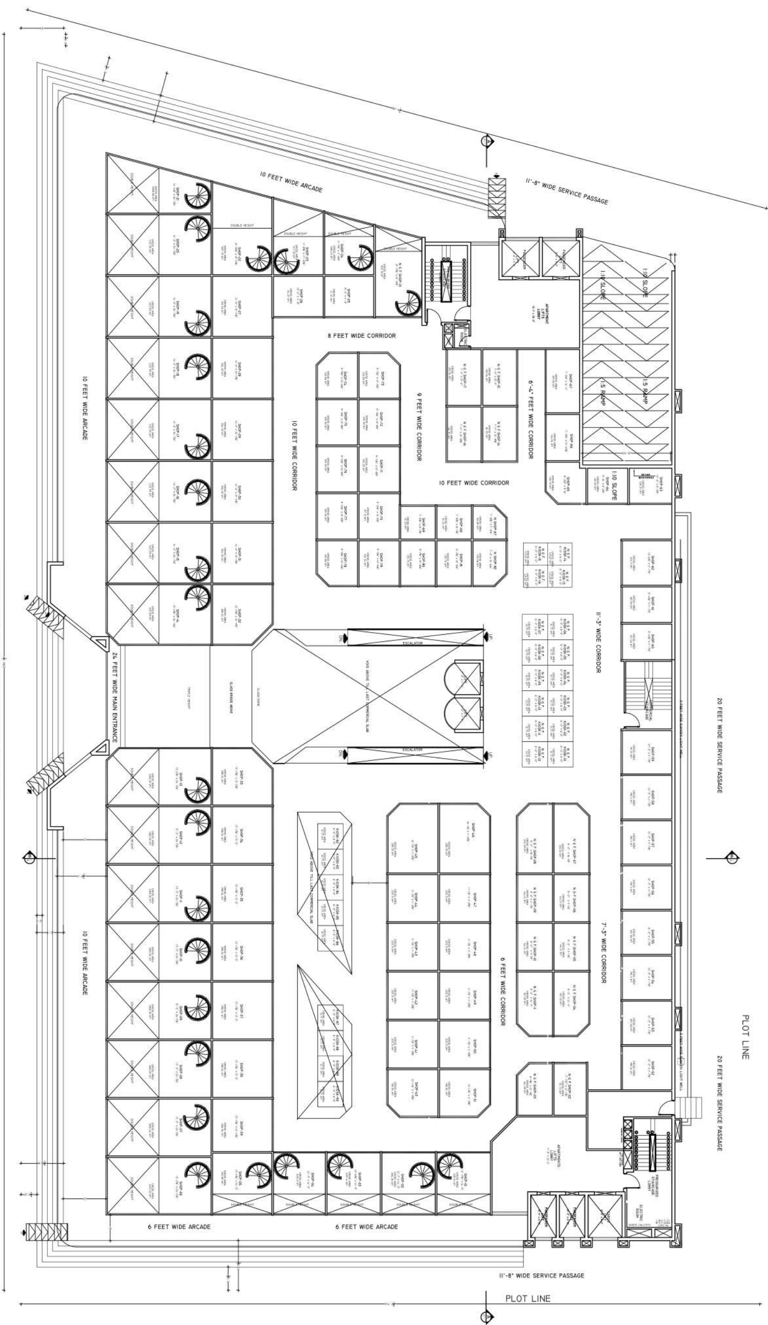
GROUND FLOOR BRANDED SHOPS WORKING PLAN AT DOWNTOWN COMMERCIAL AL-KABIR TOWN LAHORE
